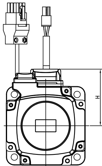
DIMENSION TABLE (MODEL WITHOUT BRAKE)
